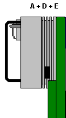
Camera without front plate, CFW10 with optical window replaces front plate, "D" block mounted to telescope side of CFW10
